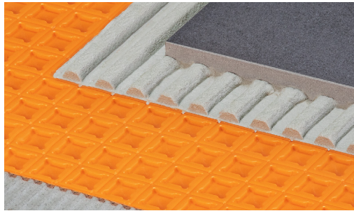
6.1 Schluter®-DITRA
