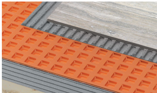
6.1 Schluter®-DITRA-XL
